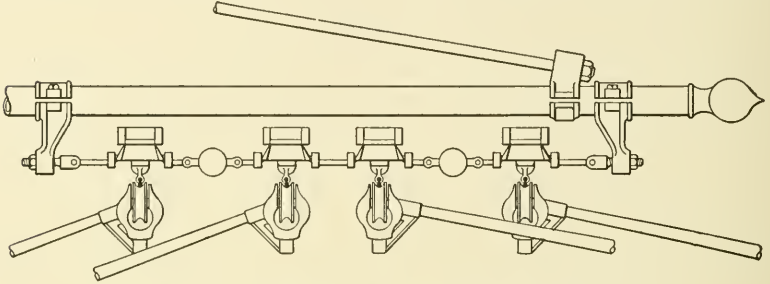
Fig. 14. Trolley Suspension Method for English Railless System
